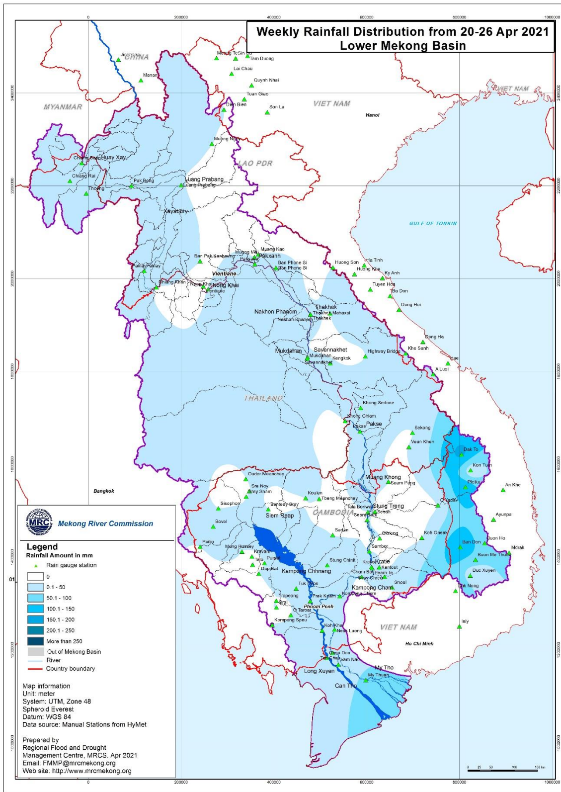
Figure 5: Weekly rainfall distribution over the LMB during 20-26 Apr 2021.
