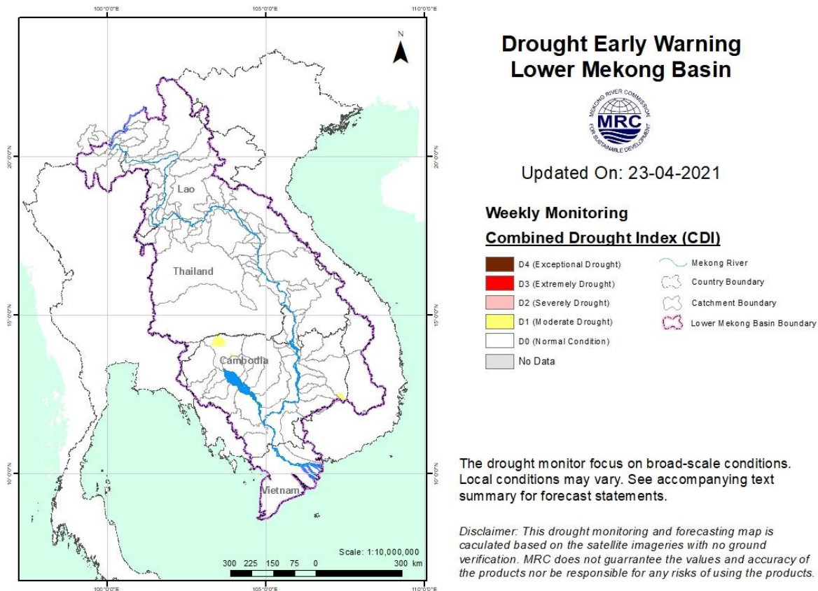
Figure 14: Weekly Combined Drought Index from 17 to 23 Apr 2021.
