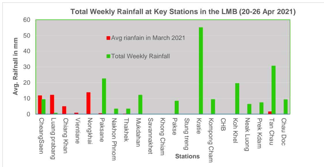
Figure 4: Weekly total rainfall at key stations in the LMB during 20-26 April 2021.
