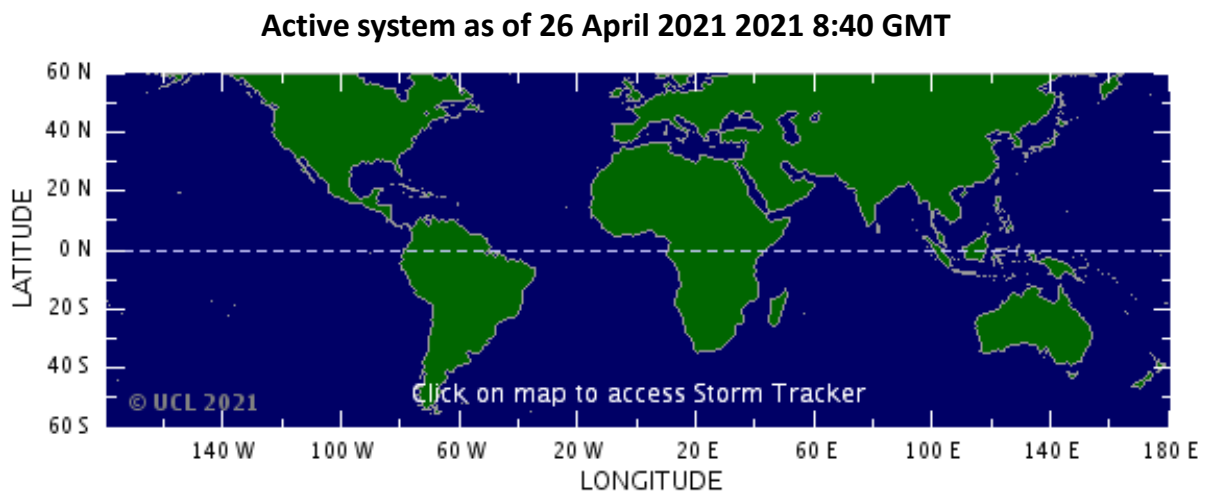
Figure 3: A Tropical Depression risk observed on 26 April 2021.
