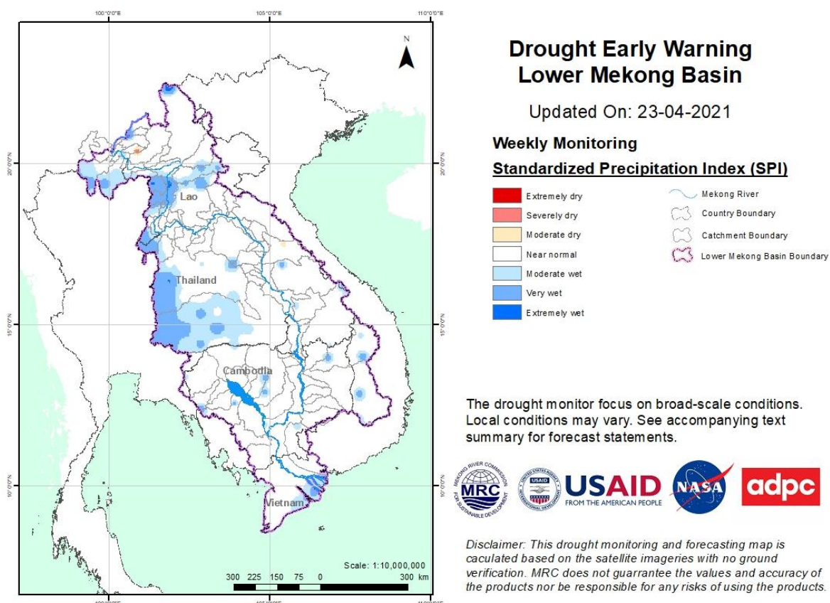
Figure 12: Weekly standardized precipitation index from 17 to 23 Apr 2021.
